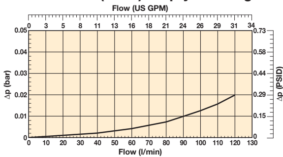
ATZ 1-120 (G1½) Empty Housing
