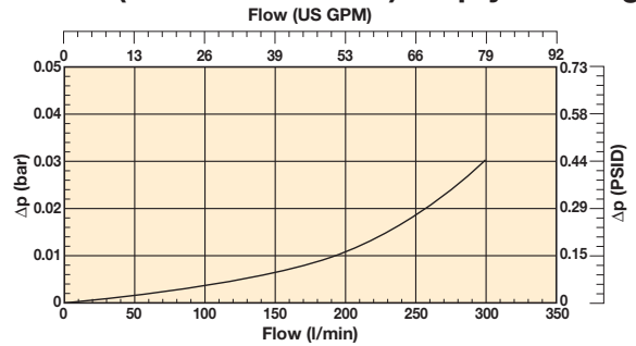
ATZ 300 (2½ SAE FLANGE) Empty Housing
