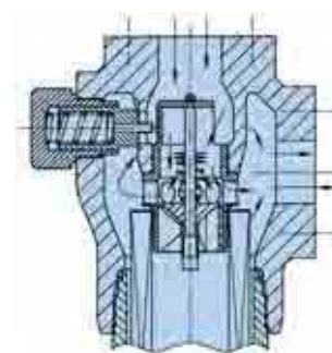
Reverse Flow Condition
